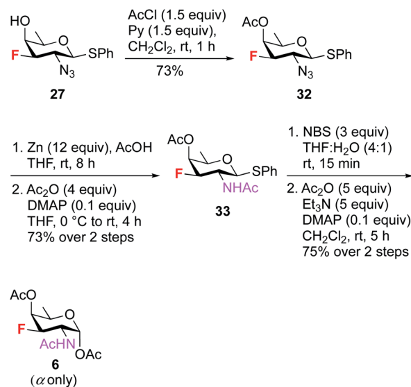
Scheme 7 Synthesis of 3F-FucNAC (F-FucNAC) 6 .
