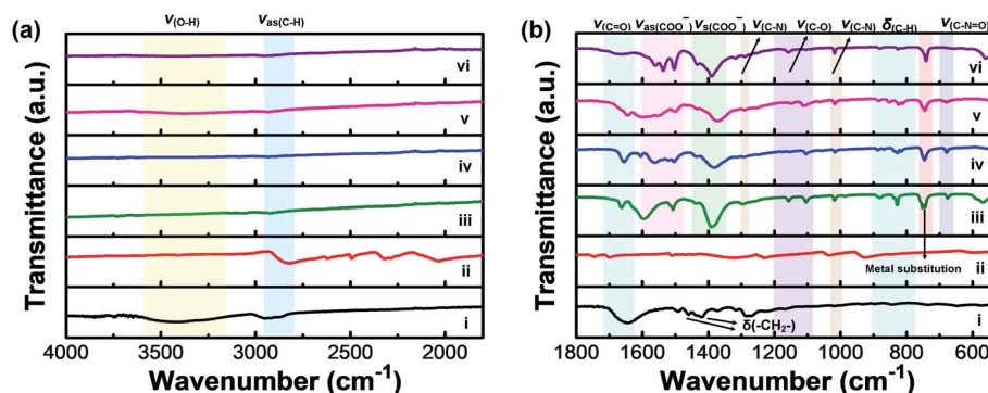
Fig. 2 FTIR spectra of (i) pure PVP, (ii) \text{H}_2\text{BDC} ligand and the as-prepared M-BDC products: (iii) Cu-BDC, (iv) Mn-BDC, (v) Ni-BDC, and (vi) Zr-BDC in the wavenumber regions of (a) 4000–1800 \text{cm}^{-1} and (b) 1800–525 \text{cm}^{-1} .
