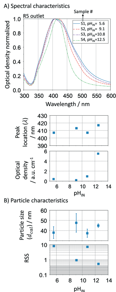
Fig. 8 Effect of initial pH (pH IN ) in the growth-stage. A. UV-vis spectra, spectral peak location and optical density at the outlet of R5; B. particle size distribution (average and standard deviation) and spherical degree (RSS). Conditions: nucleation reactor → refer to Fig. 7. 5 growth reactors → same as Fig. 6 and 7 except for changes in the pH IN .
