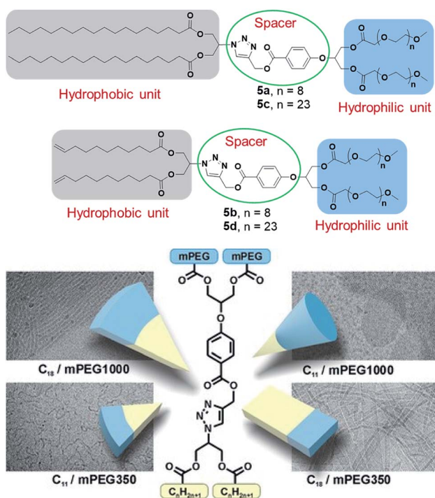
Fig. 14 Structures of twinned amphiphiles ( 5a–5d ) and geometry of aggregates along with cryo-TEM images of formed aggregates. Reprinted with permission from ref. 58. Copyright 2017 Wiley-VCH Verlag GmbH & Co. KGaA.
