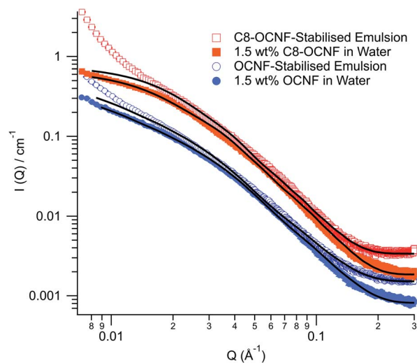
Fig. 3 SAXS patterns of 1.5 wt% OCNF (filled circles) or C8-OCNF (filled squares) and the DES in water emulsions stabilised by either 1.5 wt% OCNF (open circles) or C8-OCNF (open squares). Model fits are shown as black lines (parameters given in ESI†).
