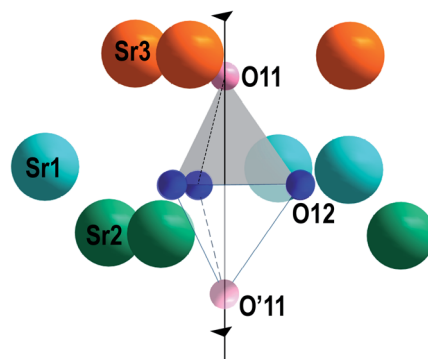
Fig. 7 The environment of \text{V1O}_4^{3-} tetrahedron by Sr1, Sr2 and Sr3 cations in \text{Sr}_9\text{In}(\text{VO}_4)_7 . Tetrahedron \text{V1O}_4^{3-} before (upper) and after (lower) rotation during the ferroelectric–paraelectric phase transition.
