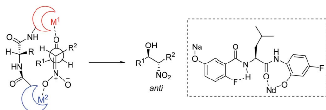
Scheme 7 Amide backbone as a platform for bimetallic complex.
