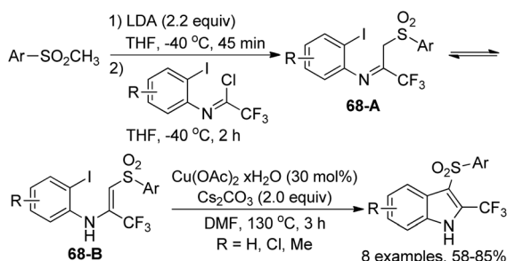
Scheme 68 Synthesis of 3-arylsulfonyl-2-trifluoromethyl-indoles.
