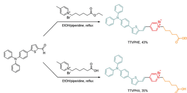
Scheme 1 The synthetic routes of TTVPHE and TTVPHA .
