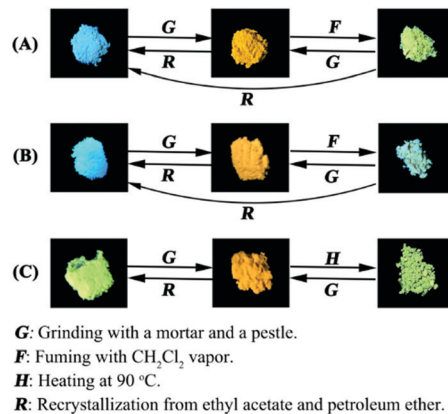
Fig. 6 Schematic diagrams of the mechanochromic behaviors of 7PTP-BPXZ (A), 5PTP-BPXZ (B) and 5,7PTP-BPXZ (C). Fluorescence images were taken under a 365 nm UV lamp.
