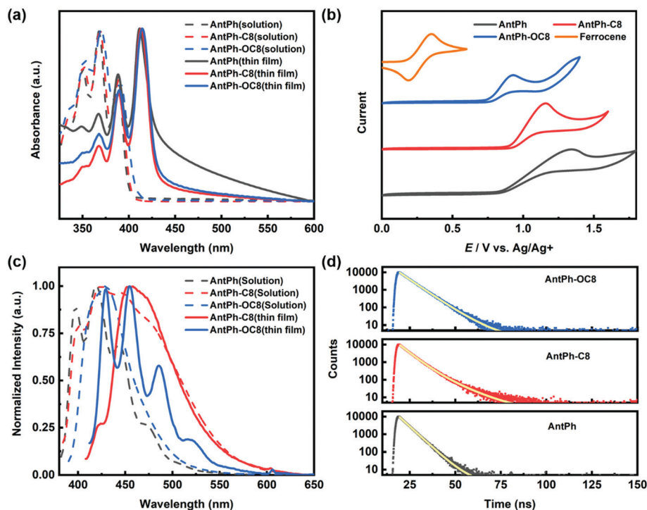
Fig. 2 UV-vis absorption spectra (a), cyclic voltammograms (b), photoluminescence spectra (c) and transient fluorescence spectra (d) of AntPh , AntPh-C8 and AntPh-OC8 in dilute CH_2Cl_2 solution and thin films. The scanning rate of the CV measurements is 0.5\text{ V s}^{-1} .
