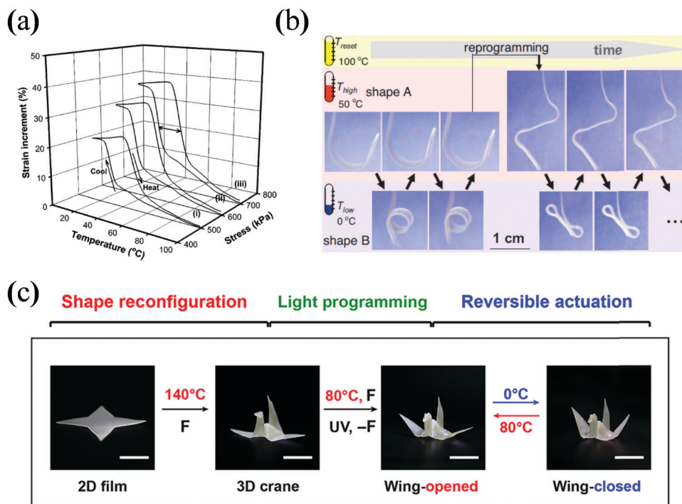
Fig. 83 2W-SME. (a) Quasi two-way shape-memory cycles under various constant stresses; (b) stress-free programmable two-way shape memory. Adapted from ref. 564, 565 and 587 with permission. Copyright (2008, 2013, and 2018) from American Chemical Society, Wiley-VCH, and AAAS.
