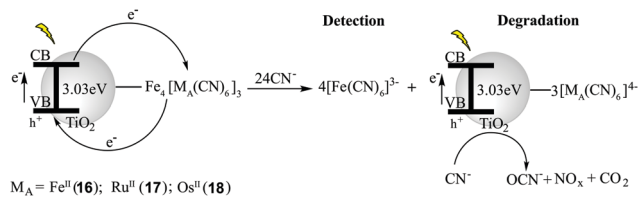
Fig. 10 The detection and degradation of CN - by 16–18 via the ICDA.
