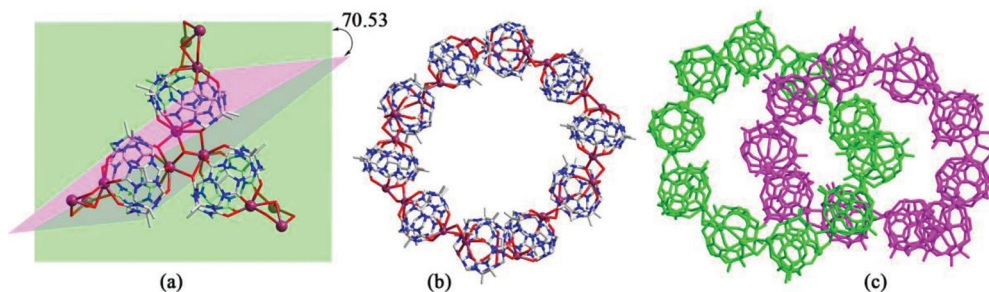
Fig. 13 (a) Schematic illustrating that the dihedral angles between any two K1 junction planes in the trigonal planar branch are identical at 70.53°. (b) A single 10-membered 1,2,4-HMeQ[5] 'bracelet'. (c) Catenation of two 10-membered 1,2,4-HMeQ[5] bracelets.
