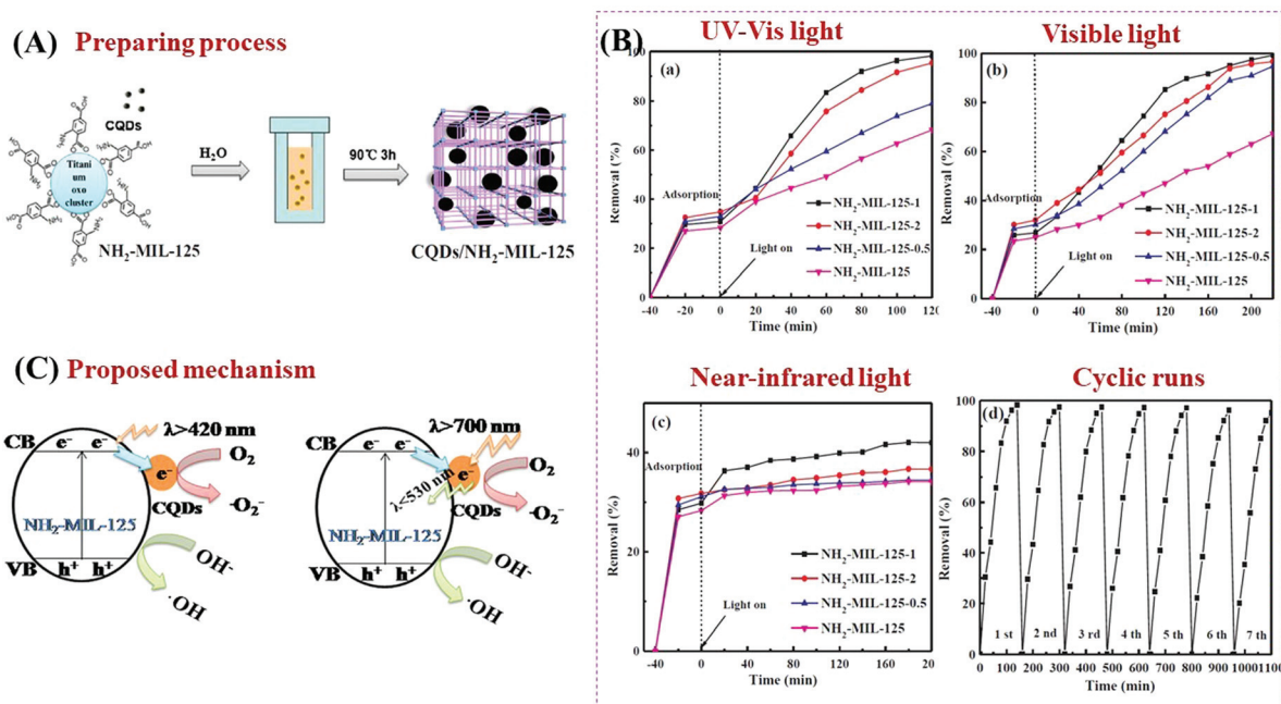
Fig. 23 (A) Schematic processes for preparing CQD/ \text{NH}_2\text{-MIL-125(Ti)} ; (B) photocatalytic degradation of RhB by \text{NH}_2\text{-MIL-125} and CQD/ \text{NH}_2\text{-MIL-125} composites under the irradiation of (a) full spectrum light, (b) visible light and (c) near-infrared light; (d) cyclic runs for RhB degradation by optimized CQD/ \text{NH}_2\text{-MIL-125} under full spectrum light; (C) proposed mechanism for charge transfer in CQD/ \text{NH}_2\text{-MIL-125(Ti)} under visible light ( \lambda > 420\text{ nm} ) and near-infrared light ( \lambda > 700\text{ nm} ) irradiation; adapted with permission from ref. 155, © 2018 Elsevier B.V.
