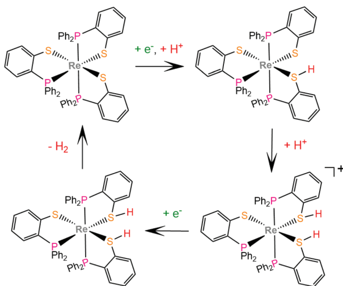
Scheme 22 (a) Molecular structures of complexes carrying diphenylphosphinobenzenethiolate ligands. (b) Proposed ligand centred mechanism catalysed by complex 50 .
