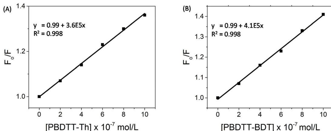
Fig. 6 (A) Stern–Volmer plots for the data from Fig. 3A and (B) Stern–Volmer plots for the data from Fig. 3B.
