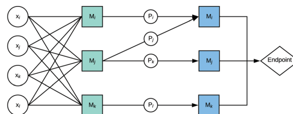
Fig. 1 The schematic representation of the structure–activity prediction networks for modeling of ENMs' toxic activity; x – descriptor that describes either structural attributes (D) or properties (P) of ENMs, M – meta-model (meta-models of the 1st layer – indicated in green, and meta-models of the 2 nd layer – indicated in blue).
