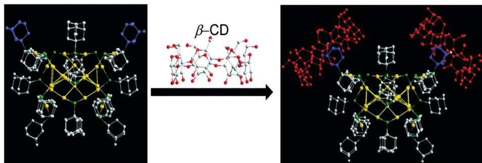
Fig. 8 Schematic illustration of formation of \text{Au}_{38}\text{S}_2(\text{SAdm})_{20}\subset(\beta\text{-CD})_2 conjugate. The host-guest interaction of \beta\text{-CD} with adamantane ligands is shown in red and blue (right side of the arrow). Other adamantane ligands are shown in white (left side of the arrow). Gold atoms are shown in yellow, sulphur atoms in green, carbon atoms in white and blue, and oxygen in red. All hydrogen atoms are omitted for clarity. Reproduced with permission. 159 Copyright 2016, Royal Society of Chemistry.
