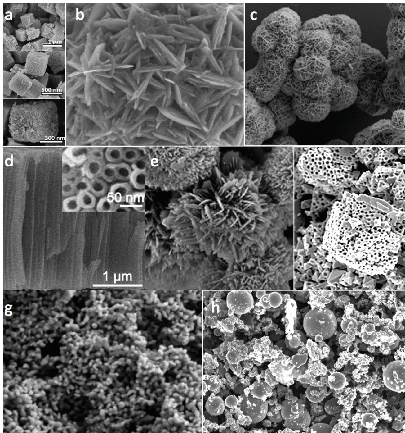
Fig. 9 Transition-metal based nano- and microstructures of: (a) \text{Co}_3\text{S}_4/\text{MoS}_2 nanocubes (adapted from ref. 328), (b) \text{CoS} nanoflakes (adapted from ref. 334), (c) \text{Cu}_7\text{S}_4/\text{CuS} nano-hollows (adapted from ref. 337), (d) \text{TiS}_2 nanorods (adapted from ref. 339), (e) \text{VSe}_2 nanoflakes (adapted from ref. 340), (f) \text{Cu}_2\text{O} nanosponges (adapted from ref. 341), (g) \text{La}_{0.7}\text{Ca}_{0.3}\text{MnO}_3 nanospheres (adapted from ref. 342) and (h) \text{CuTa}_{10}\text{O}_{26} nanoplates (adapted from ref. 343).
