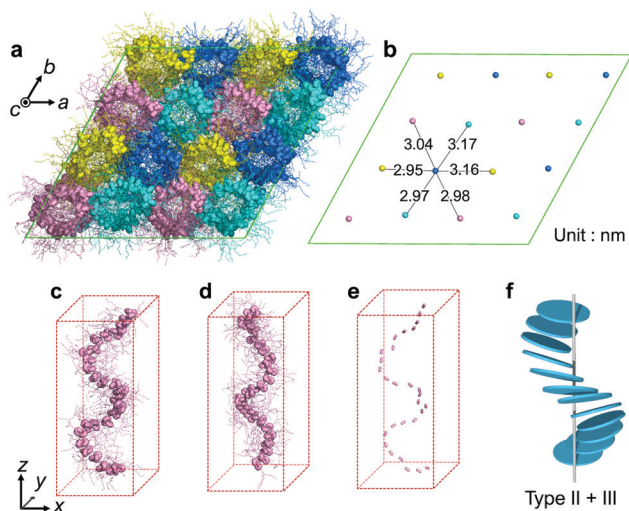
Fig. 4 (a) Top view of M\text{-}\Delta\text{-Ru-C8} after 200 ns of MD simulation. The Ru core and peripheral groups in each mesogen molecule are represented by spheres and sticks, respectively. (b) Average positions of Ru atoms in each column. (c) Side view of a single column in M\text{-}\Delta\text{-Ru-C8} . (d) Side view of a single column in P\text{-}\Lambda\text{-Ru-C8} . (e) The C_3 axis of each mesogen in (c) is displayed. (f) Schematic of a single-column structure in M\text{-}\Delta\text{-Ru-C8} , corresponding to a hybrid of types II and III.
