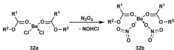
Scheme 6 Displacement of chlorido by nitrate ligands in beryllium esters. \text{R}^1 = \text{H, Me; R}^2 = \text{Me, Et, } ^i\text{Pr} . 92
