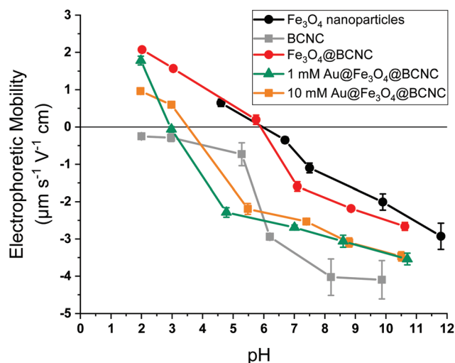
Fig. 3 Electrophoretic mobility of bare \text{Fe}_3\text{O}_4 nanoparticles, BCNCs, \text{Fe}_3\text{O}_4 @BCNCs, 1 mM and 10 mM \text{Au@Fe}_3\text{O}_4 @BCNCs in 0.01 M NaCl solution. The error bars indicate standard deviation of three measurements.
