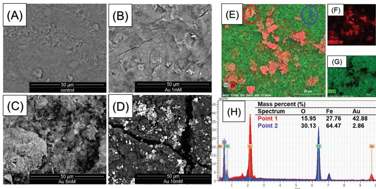
Fig. 2 Backscattered SEM images of the aggregated (A) \text{Fe}_3\text{O}_4 @BCNCs, (B) 1 mM \text{Au@Fe}_3\text{O}_4 @BCNCs, (C) 5 mM \text{Au@Fe}_3\text{O}_4 @BCNCs and (D) 10 mM \text{Au@Fe}_3\text{O}_4 @BCNCs. EDS mapping of (E) 10 mM \text{Au@Fe}_3\text{O}_4 @BCNCs with (F) Au and (G) Fe elements highlighted. The corresponding (H) EDS spectra of the map are provided with mass percent of O, Fe, and Au shown.
