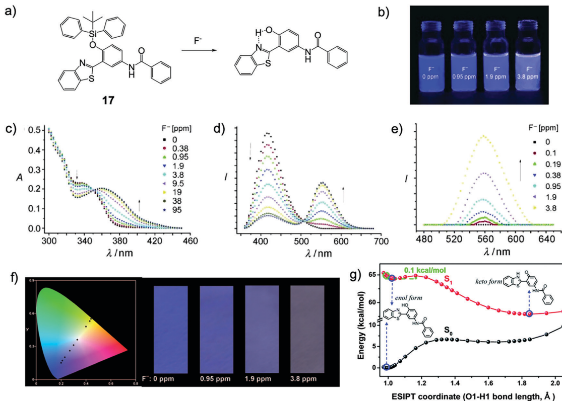
Fig. 7 Sensing mechanism and performance of 7 . (a) Reaction scheme of 7 with \text{F}^- . (b) Pictures of dispersions of 7 upon addition of NaF under a UV lamp. (c) Absorption and (d) and (e) fluorescence spectra of the dispersions of 7 200 s after addition of NaF, \lambda_{\text{ex}} = 350 nm (d) and 385 nm (e). (f) CIE 1931 ( x, y ) chromaticity diagram of the test papers for the detection of NaF at different concentrations derived from the fluorescence spectra (black circles); NaF concentration from left to right: 0, 0.38, 0.95, 1.9, 3.8, 9.5, 19, 38, and 95 ppm (left); images of the test papers after immersion into solutions with different concentrations of NaF (right). Reproduced with permission from ref. 29. Copyright 2010, John Wiley and Sons. (g) The calculated potential energy curve of the \text{S}_1 state for the desilylated product of 7 computed by the TDDFT/B3LYP/TZVP method. The energies of the \text{S}_0 state were calculated under the geometries of the corresponding \text{S}_1 state. Reproduced with permission from ref. 30. Copyright 2014, Royal Society of Chemistry.
