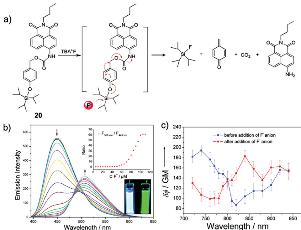
Fig. 9 Sensing mechanism and performance of 20 . (a) Reaction scheme of 20 with TBAF. (b) Fluorescence spectra of 20 (10 \mu M) in \text{CH}_3\text{CN} in the presence of TBAF (0–110 \mu M). Insets: (upper) Ratios of fluorescent intensities at 508 and 449 nm as a function of \text{F}^- concentration; (lower) fluorescence images of 20 (10 \mu M) before and after addition of TBAF (110 \mu M) in \text{CH}_3\text{CN} . \lambda_{\text{ex}} = 365 nm. (c) Two-photon action spectra of 20 (10 \mu M solution in \text{CH}_3\text{CN} ) before (blue line) and after (red line) addition of TBAF (110 \mu M). Error bars represent the standard deviation from replicate experiments ( n = 10 ). Reproduced with permission from ref. 39. Copyright 2011, American Chemical Society.
