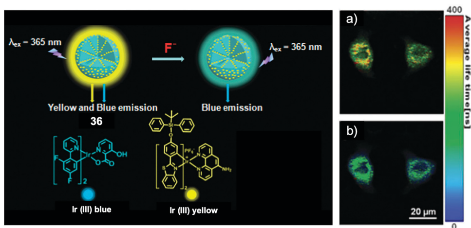
Fig. 19 Schematic of ratiometric nanosensor 36 and in vitro imaging. Phosphorescence lifetime images ( \lambda_{\text{ex}} = 405 nm) of HepG2 cells incubated with the nanosensor (a) before and (b) after treatment with 15 \mu\text{M} of NaF. Reproduced with permission from ref. 72. Copyright 2015, Royal Society of Chemistry.
