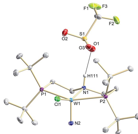
Fig. 3 Molecular structure of \mathbf{9}^{\text{OTf}} in the crystal obtained by single crystal X-ray diffraction. Hydrogen atoms are omitted for clarity except H111.
