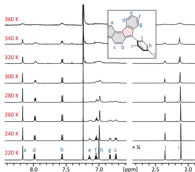
Fig. 4 Temperature-dependent ^1\text{H} NMR spectra of 2 ( \text{CDCl}_3 , 600 MHz). The signals were assigned at 220 K using 2D spectroscopic methods (see the ESI † ).
