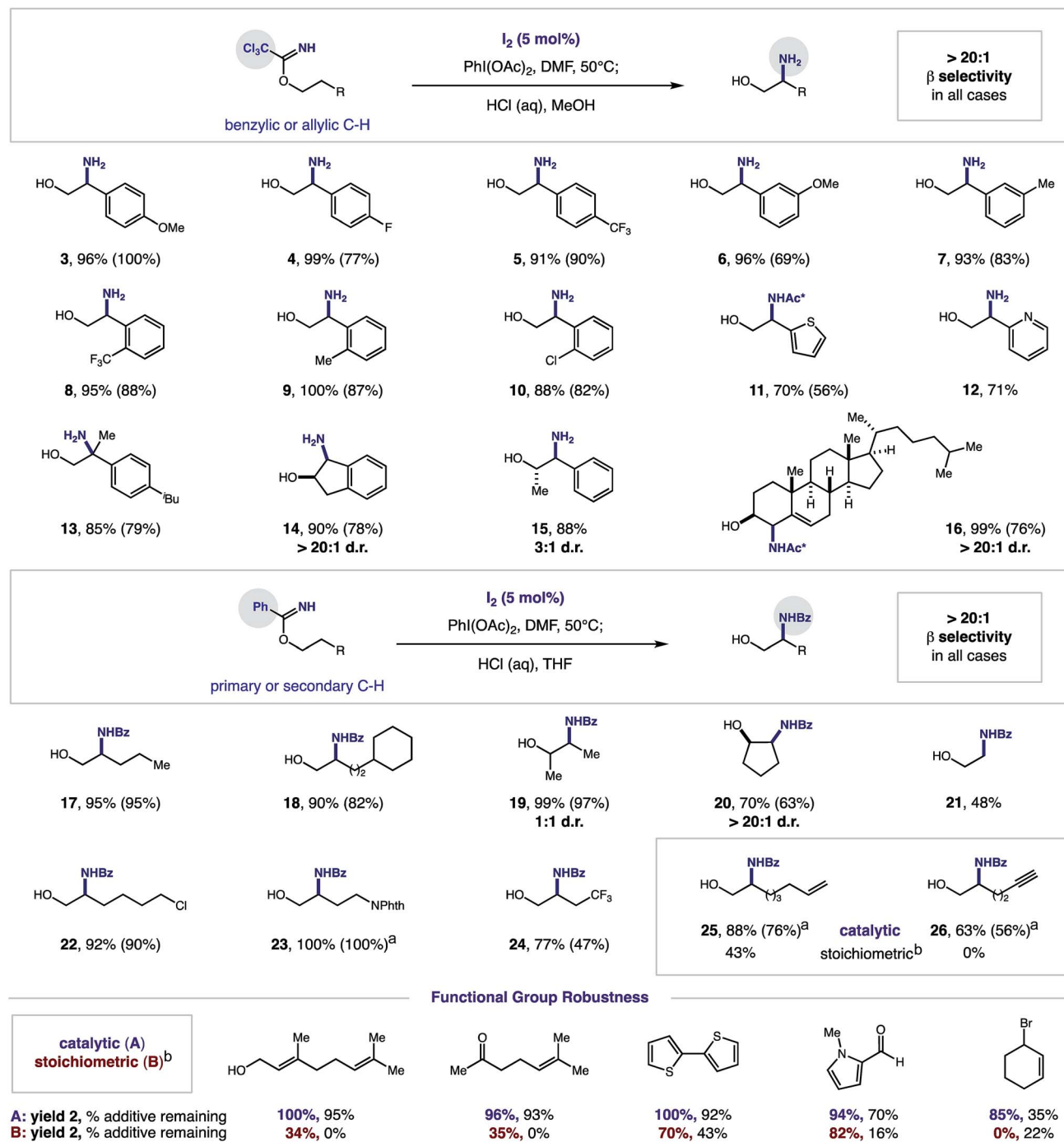
Fig. 3 Synthetic utility of iodine-catalyzed \beta C–H amination of imidates. Conditions : 0.4 mmol imidate, \text{I}_2 (5 mol%), PhI(OAc) 2 (1.2 equiv.), DMF (0.2 M), 50 °C. 1 H NMR yield of oxazoline determined vs. standard. Hydrolysis with HCl (2 M) affords amino alcohol (isolated yield, in parenthesis). a Isolated yield of oxazoline. b Stoichiometric NaI (ref. 12). Ac* refers to trichloroacetamide. Functional group robustness : C–H amination yield, % additive remaining.
