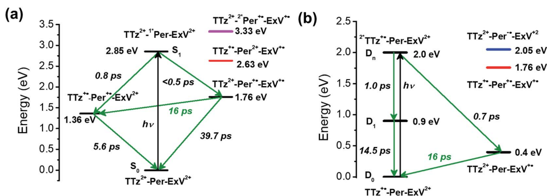
Fig. 5 Energy level diagrams of (a) \text{Per} \subset \text{TTzExVBox}^{4+} and (b) \text{Per} \subset \text{TTzExVBox}^{3+} in \text{CH}_3\text{CN} , in which the zero energy level is taken to be the \text{Per S}_0 state in (a) and the \text{TTz}^{2+} \text{D}_0 state in (b), respectively. The ICT pathways from \text{ExV}^{2+} to \text{TTz}^{2+} as well as the corresponding timescales are highlighted in red. The states involved in superexchange mixing are shown in red, blue, and magenta.
