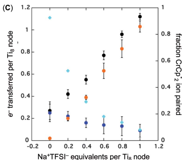
Fig. 2 Reduction of MIL-125 with \text{CrCp}_2^* and \text{Na}^+ ( \text{NaTFSI} ). (A) Schematic of the reaction. (B) ^1\text{H} NMR spectra ( d_8 -THF + \text{CD}_3\text{CN} 4 : 1 v/v) of mixtures of MIL-125 + 3 equiv. \text{CrCp}_2^* + different equiv. of \text{Na}^+ per \text{Ti}_8 node: 0 (red), 0.2 \text{Na}^+ (yellow), 0.4 \text{Na}^+ (green), 0.6 \text{Na}^+ (light blue), 0.8 \text{Na}^+ (dark blue), and 1.0 \text{Na}^+ (purple). (C) Plot of e^- transferred to MIL-125 (left axis) and fraction of \text{CrCp}_2^* ion-paired in reduced MIL-125 (right axis) versus equiv. \text{NaTFSI} added. Orange circles: equiv. of \text{Na}^+ associated with the reduced MIL-125, derived from the \text{CrCp}_2^{*0/+} chemical shift. Blue circles: equiv. \text{CrCp}_2^* associated with the reduced MIL-125, derived from the change in integration of the \text{CrCp}_2^{*0/+} resonance upon mixing with MIL-125. Black circles: total extent of reduction (the sum of the blue and orange circles). Light blue diamonds: fraction of the reduced MIL-125 that is associated with \text{CrCp}_2^* .
