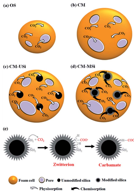
Fig. 7 Proposed mechanisms of CO 2 adsorption for the (a) OS, (b) CM, (c) CM-USi and (d) CM-MSi foams, and (e) chemisorption between CO 2 and modified silica in CM-MSi foam.
