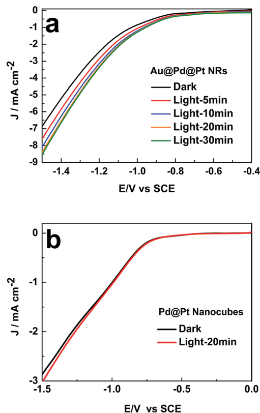
Fig. 4 Influence of the illumination time on the LSV curves of (a) 49 nm Au@Pd@Pt NRs and (b) Pd@Pt nanocubes in 0.1 M \text{KHCO}_3 (pH = 6.8) \theta_{Pt} = 0.5 ; scan rate: 50 \text{mV s}^{-1} .
