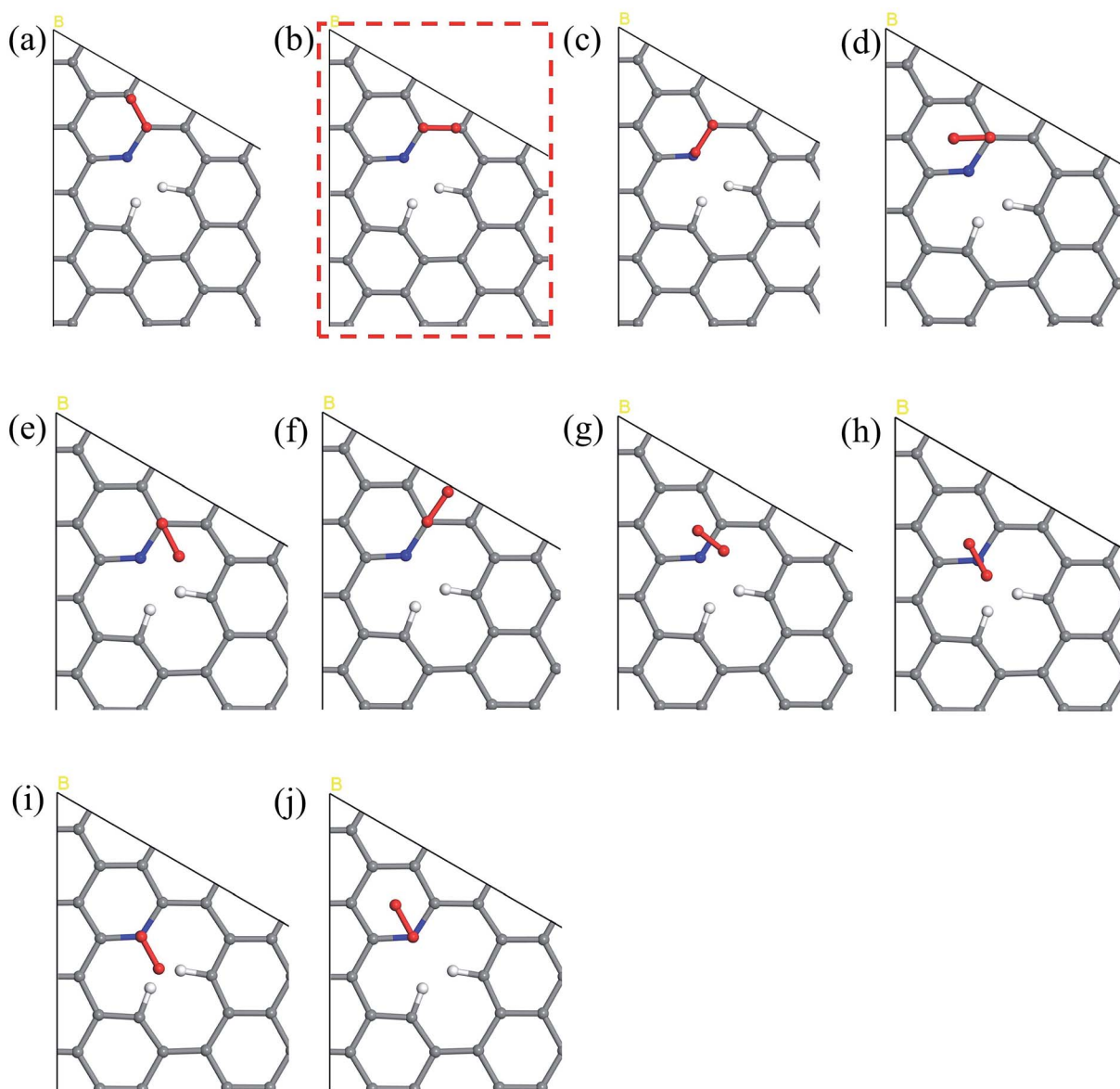
Fig. 2 The potential sites where \text{O}_2 can be located on the N6 substrate for the first step of the ORR. N6_S1_(a) CBC1 (b) CBC2 (c) CBN (d) CH1 (e) \text{CH}_2 (f) \text{CH}_3 (g) HBH (h) HNH (i) NH1 and (j) \text{NH}_2 . The model marked by red dashed line has the lowest energy upon geometry optimization, indicating the most likely adsorption configuration and is used in the free energy diagram.
