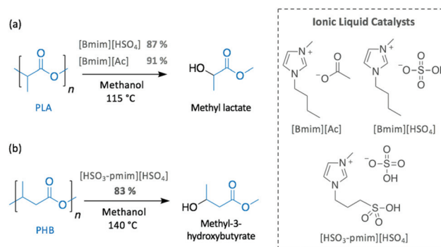
Scheme 9 PLA and PHB depolymerisation using ILs.
