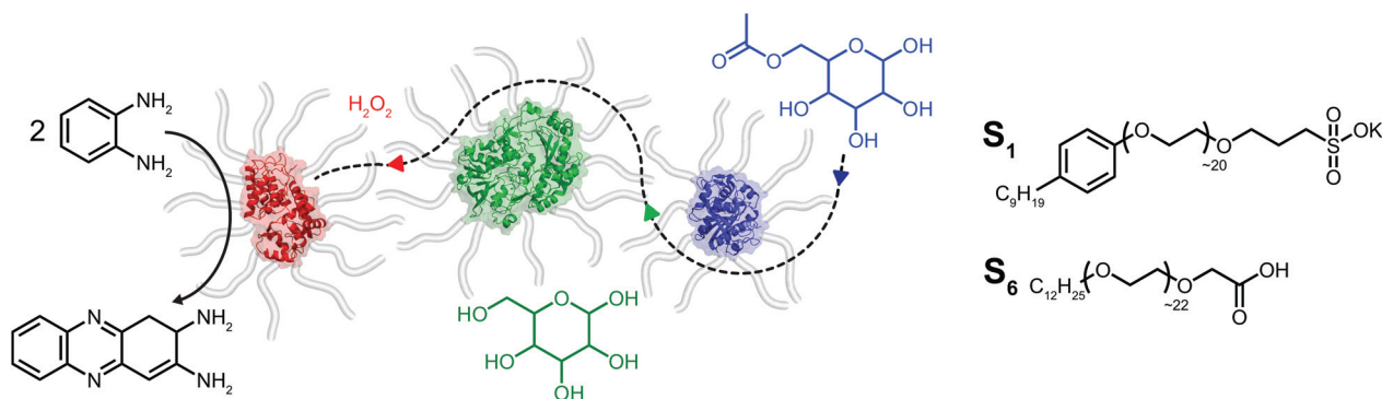
Fig. 1 Chemical structures of polymer surfactants poly(ethylene glycol)-4-nonylphenyl-3-sulfopropyl ether (S 1 ) and carboxylated Brij-L23 (S 6 ) which are used in the production of solvent-free protein polymer hybrid nanoconjugates. Biohybrids produced from the three enzymes horseradish peroxidase (red), glucose oxidase (green), and Thermomyces lanuginosus lipase (blue) are utilized for constructing enzymatic cascades in the solvent-free phase. The enzyme-specific substrates acetylated glucose, glucose, and hydrogen peroxide are indicated in blue, green and red, respectively. Horseradish peroxidase biohybrid-mediated formation of 2,3-diaminophenazine from the o -phenylenediamine substrate is shown in black. The efficient diffusion, turnover and release of species is represented schematically by the dotted line.
