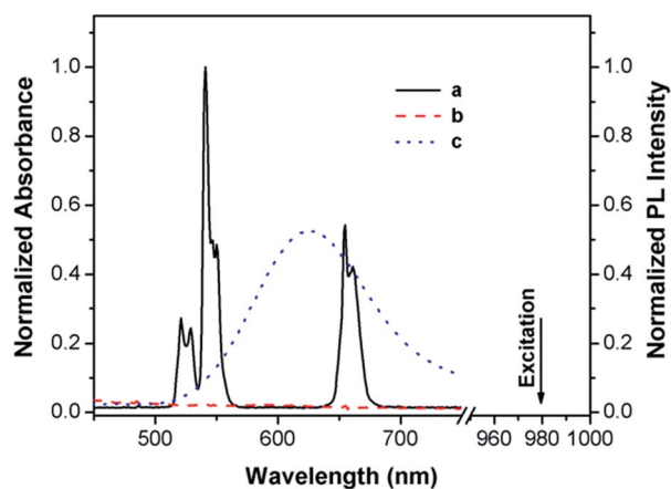
Fig. 2 UCL spectrum of DSPC-coated \text{NaYF}_4\text{:}20\%\text{Yb},2\%\text{Er} (DSPC-UCNPs) under excitation from a 980 nm laser (a), and UV-vis spectra of the protein apo-azurin in the absence (b) and presence of \text{Cu}^{2+} (c).
