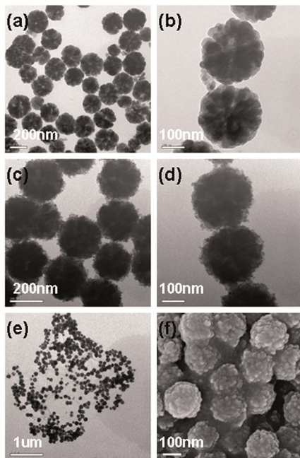
Fig. 17 TEM images of the products at different stages (a and b) p\text{Fe}_3\text{O}_4 , (c and d) p\text{Fe}_3\text{O}_4@Z\text{nO} , (e) \text{GN}p\text{Fe}_3\text{O}_4@Z\text{nO} , and (f) corresponding FE-SEM image 181 – reproduced by permission of the Royal Society of Chemistry.
