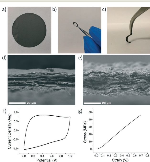
Fig. 4 Digital images of (a) an rGO electrode and (b and c) an rGO/ANF composite electrode (no CNTs). Cross-sectional SEM images of (d) an rGO/ANF electrode without CNTs (95/5 wt% rGO/ANFs) and (e) with 20 wt% CNTs (76/4/20 wt% rGO/ANFs/CNTs). (f) A representative cyclic voltammogram and (g) a typical stress–strain curve for an rGO/ANF/CNT composite electrode (90.25 wt% rGO, 4.75 wt% ANFs, 5 wt% CNTs).
