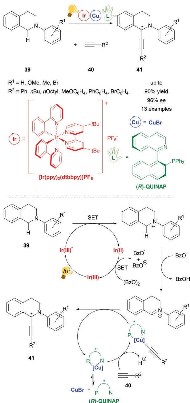
Scheme 16 Asymmetric alkynylation of tetrahydroisoquinoline (THIQ) via photoredox catalysis, overview (top) and mechanism (bottom). Reagents and conditions: alkyne 40 (1.50 equiv.), Ir-photocat. (1.0 mol%), Cu salt (10.0 mol%), ( R )-QUINAP (15.0 mol%), (BzO) 2 (1.20 equiv.), THF/MeCN (1/1), -20 °C, Ar, visible light (26 W), 2 d. 73
