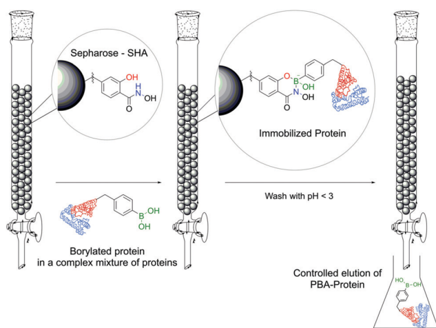
Fig. 25 PBA-modified proteins can be selectively immobilized and purified on a SHA-Sephacryl resin.
