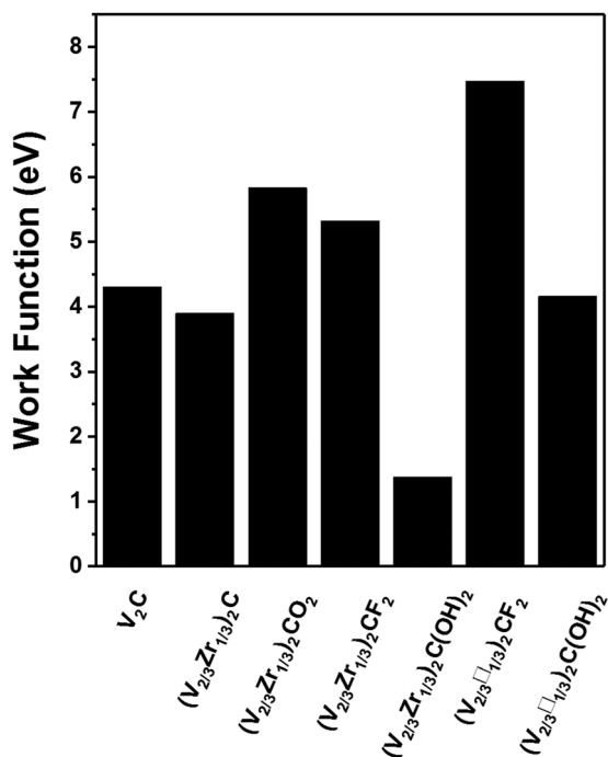
Fig. 5 Work functions of V_2C , pristine (V_{2/3}Zr_{1/3})_2C , bimetallic (V_{2/3}Zr_{1/3})_2CO_2 and vacancy-ordered (V_{2/3}\square_{1/3})_2CO_2 MXenes.
