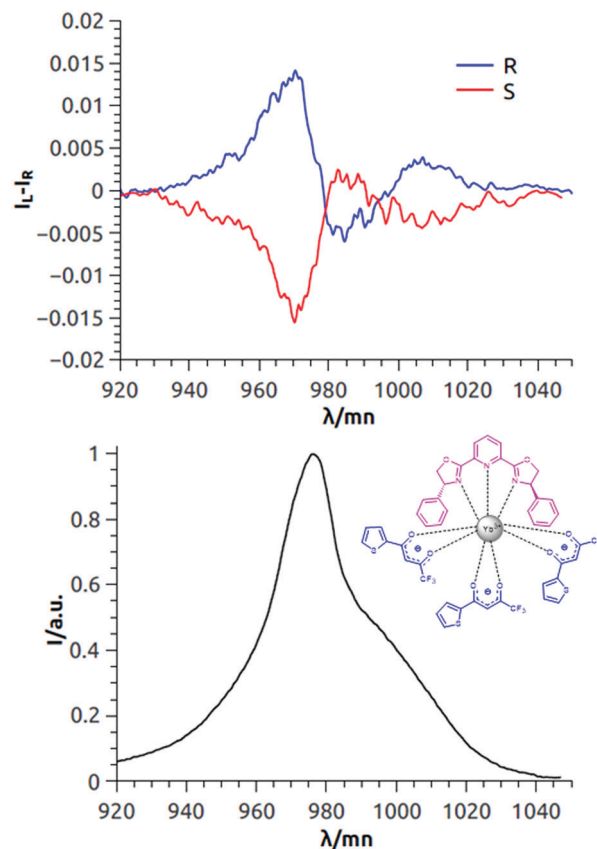
Fig. 2 Top: NIR-CPL spectra of both the enantiomers of \text{Yb}(\text{TTA})_3^1\text{PhPyBox} ; bottom: total NIR emission. The spectra are measured in 6 mM \text{CH}_2\text{Cl}_2 solution under 365 nm irradiation (room temperature).
