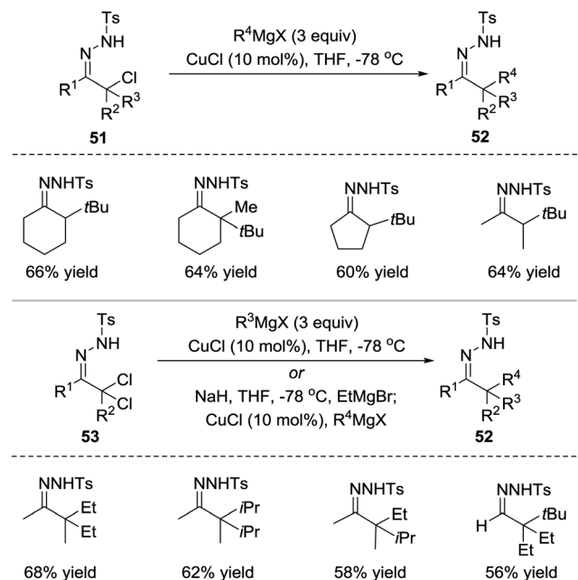
Scheme 23 Cu(I)-Catalyzed conjugate addition of Grignard reagents to azoalkenes.
