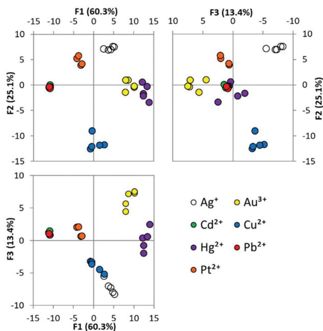
Fig. 3 LDA score plot for the analysis of seven metal ions performed in quintuplicate (100 \mu\text{M} metal ion, pH 7.4, 20 mM HEPES) describing the response to thiocoumarin 545 in ethanol, isopropanol, acetonitrile and DMSO. Each pairing of the three main factors is plotted in a separate 2D plot.
