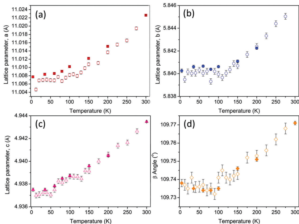
Fig. 4 Lattice parameters (a) a , (b) b , (c) c , and (d) \beta angle as a function of temperature showing a invariant effect in the lattice b -direction and \beta angle which persists up to a temperature of approximately 130 K. Open and closed symbols are XRD and neutron diffraction data respectively. Note: error bars indicate 1 standard deviation and in some data are smaller than the symbol size.
