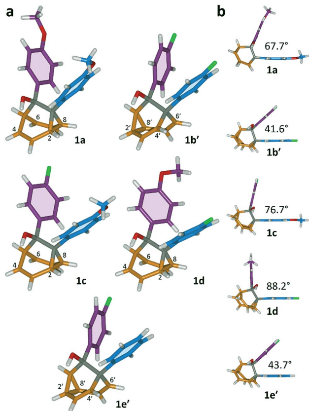
Fig. 3 X-ray crystal structures of 1/1' shown in stick representations. † (a) Whereas the major solution-phase valence isomers are obtained in some cases ( 1a , 1c and 1d ), the minor solution-phase isomers crystallise preferentially in others ( 1b' and 1e' ). (b) Side-on views show the variation in dihedral angles between the planes of the aromatic rings. Selected interatomic distances at 120 K (Å): 1a , C2–C8 1.592(2), C4...C6 2.359(2); 1b' , C2'–C8' 1.592(3), C4'...C6' 2.353(2); 1c , C2–C8 1.582(2), C4...C6 2.364(2); 1d , C2–C8 1.586(2), C4...C6 2.367(2); 1e' , C2'–C8' 1.591(2), C4'...C6' 2.345(2). Oxygen atoms are shown in red, fluorine atoms are green, hydrogen atoms are white, and carbon atoms are blue, purple, orange or grey.
