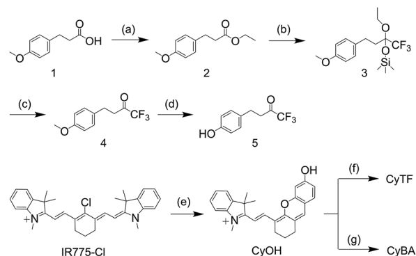
Scheme 2 Synthetic route of CyTF and CyBA. (a) H 2 SO 4 (con.), reflux, 4 h, EtOH, 97%; (b) TMS-CF 3 , CsF, THF, 18 h, 86%; (c) TBAF, THF, 5 h, then 4 M HCl, 3 h, 97%; (d) BBr 3 , -78 °C, room temperature, 12 h, CH 2 Cl 2 , 74%; (e) K 2 CO 3 , resorcinol, CH 3 CN, 2 h; (f) 5, BTC, Et 3 N, 0 °C, 2 h, CH 2 Cl 2 , 28%; (g) 4-methylphenylboronic acid pinacol ester, K 2 CO 3 , CH 3 CN, 75%.
