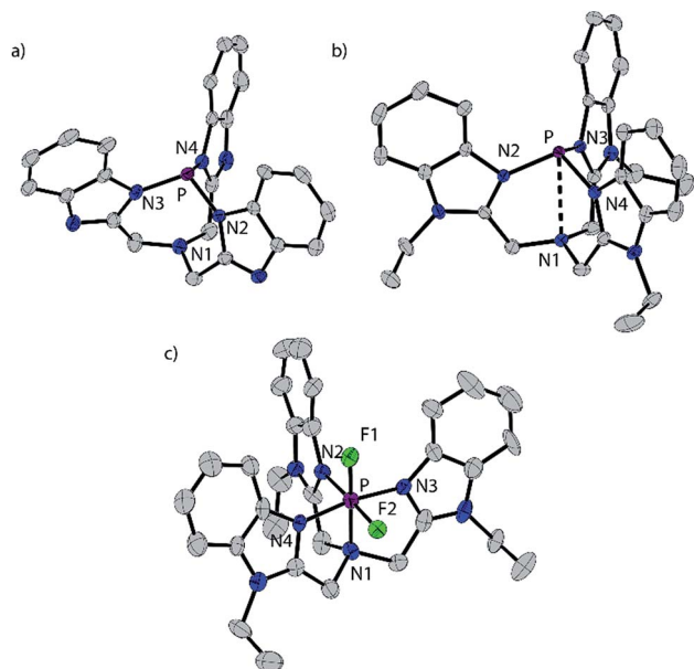
Fig. 1 Solid state structures of one of two independent molecules of P(BIM) (a), the cation in [\text{P}(\text{BIMeT}_3)]^{3+} (b), and cation in [\text{PF}_2(\text{BIMeT}_3)]^{3+} (c). Thermal ellipsoids are shown at a 50% probability level. Hydrogen atoms, solvent molecules and triflate anions are omitted for clarity. Inter-atomic distances and angles are summarized in Table 2.
