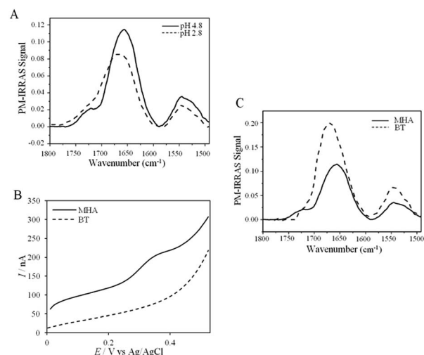
Fig. 5 AcoP behavior on SAMs. (A) PMIRRAS spectrum of AcoP at 20 \mu\text{M} adsorbed for 1 h on MHA-Au in 10 mM \text{NH}_4\text{AC} at pH 4.8 (solid line) and pH 2.8 (dashed line); (B) SWVs of AcoP adsorbed on MHA (solid line) or BT (dashed line) in 10 mM \text{NH}_4\text{AC} at pH 4.8; (C) PMIRRAS spectra of AcoP at 20 \mu\text{M} in 10 mM \text{NH}_4\text{AC} at pH 4.8 adsorbed for 1 h on MHA-Au (solid line) or BT-Au (dashed line).
