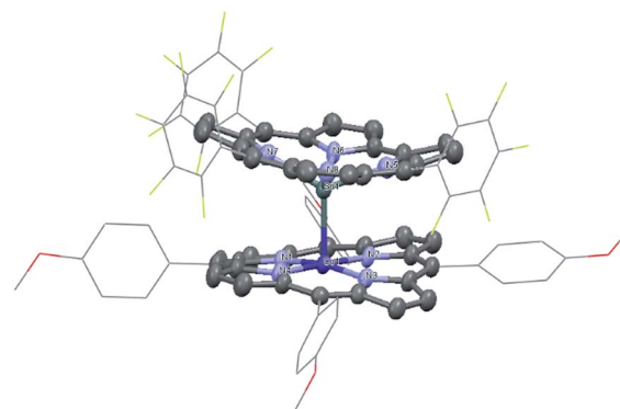
Fig. 1 Solid state structure of 1. Hydrogen atoms are omitted for clarity. Selected bond lengths (Å): Sn1-Co1 2.4559(10), Sn1-N5 2.120(5), Sn1-N6 2.107(5), Sn1-N7 2.122(5), Sn1-N8 2.108(5), Co1-N1 1.957(4), Co1-N2 1.960(5), Co1-N3 1.967(4), and Co1-N4 1.955(5).
