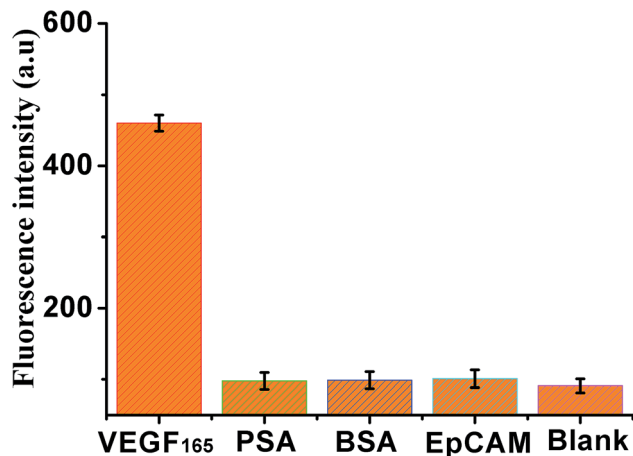
Fig. 5 Fluorescence intensity (at an emission wavelength of 519 nm) of the sensor in the presence of VEGF 165 (10 ng mL -1 ), PSA (100 ng mL -1 ), BSA (100 ng mL -1 ), EpCAM (100 ng mL -1 ) and black, respectively. Error bars: SD, n = 3 .
